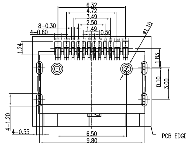
PCB LAYOUT TOLERANCESIZE:±0.05
