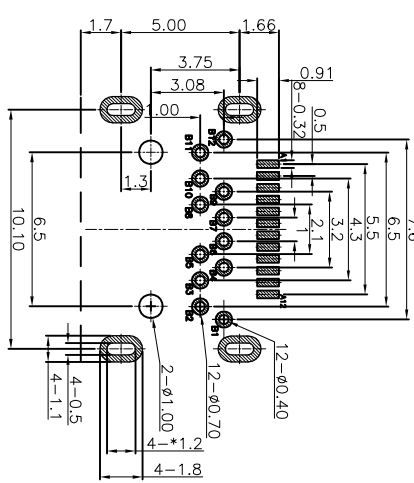
RECOMMENDED PCB LAYOUT Tolerance: ±0.05mm
