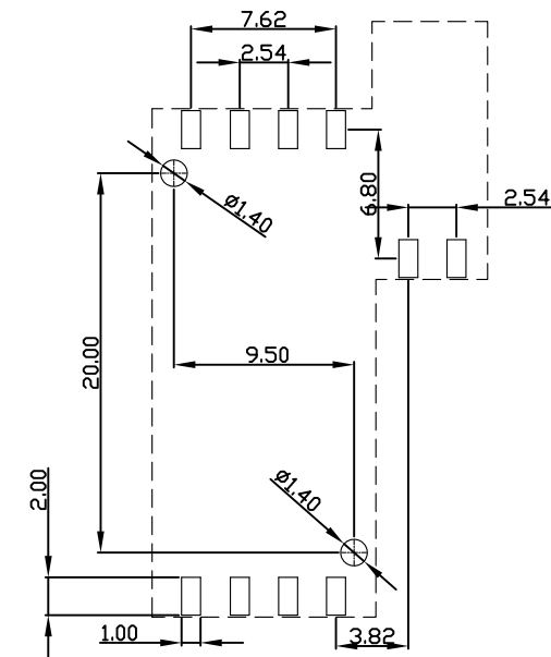
Recommended PCB LAYOUT TOL.:±0.05
